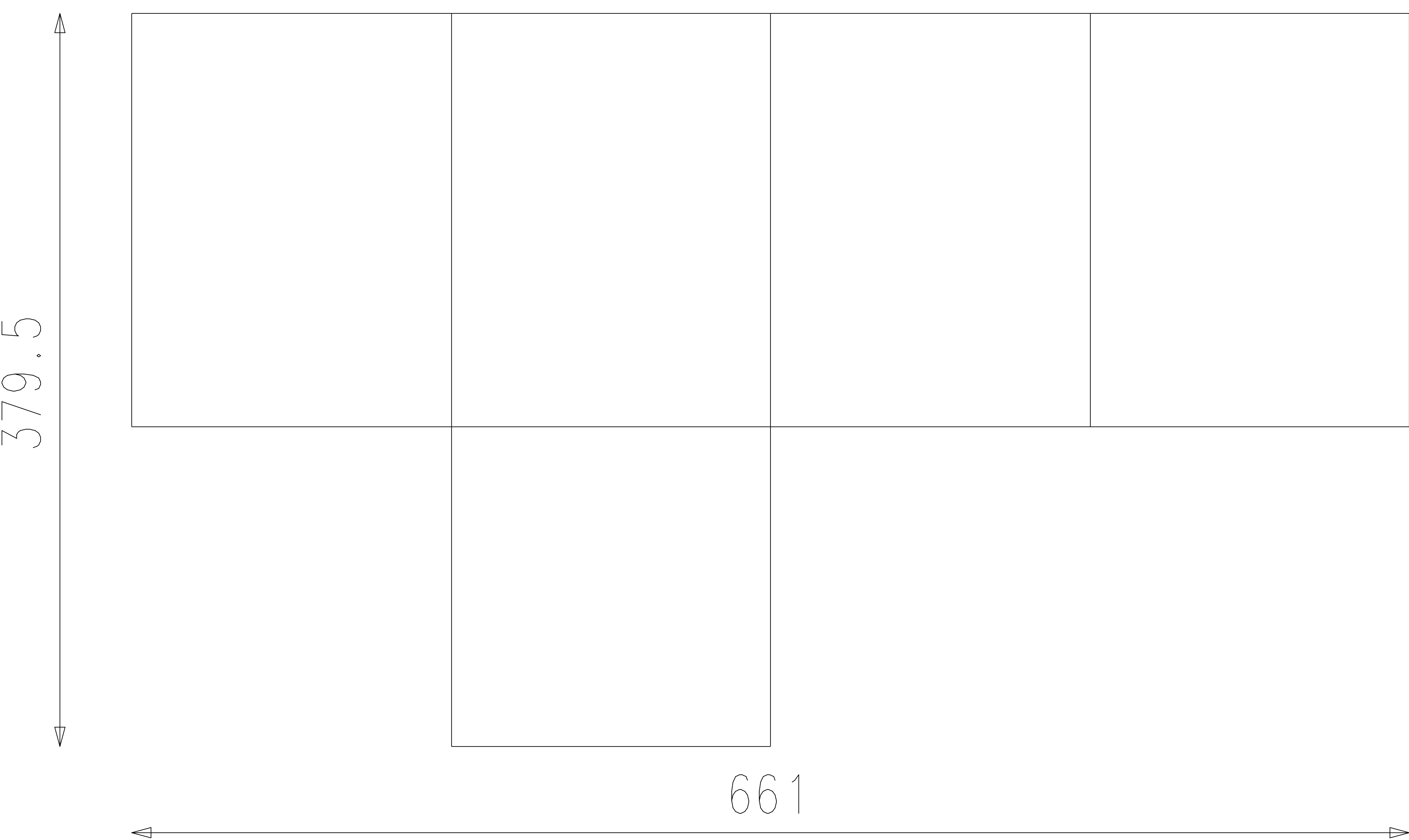
SLEEVE RIGID
